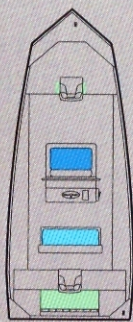
MV 1860 AW Special 18' Length 60" Bottom/86" Width 90 HP maximum Weight: 780# Hull thickness: .102" Capacity: 6 persons
