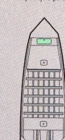
MV 1544 AW DD Tunnel 15' Length 46" Bottom/65" Width 25 HP maximum Weight: 260# Hull thickness: .082" Capacity: 4 persons
