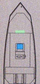
V-Bow 1650 AW Tunnel CC 16' Length 50" Bottom/74" Width 60 HP maximum Weight: 585# Hull thickness: .102" Capacity: 5 persons
