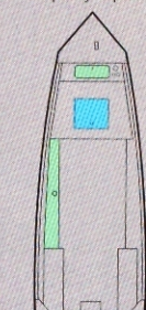
Waterfowler 15 15' Length 46" Bottom/65" Width 25 HP maximum Weight: 330# Hull thickness: .082" Capacity: 4 persons
