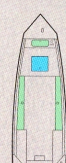
Waterfowler 16 16' Length 50" Bottom/74" Width 40 HP maximum Weight: 525# Hull thickness: .102" Capacity: 5 persons
