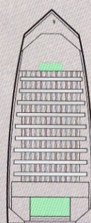
MV 1860 AW 18' Length 60" Bottom/86" Width 90 HP maximum Weight: 780# Hull thickness: .102" Capacity: 6 persons
