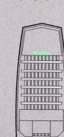
MV 1450 AW 14' Length 50" Bottom/74" Width 30 HP maximum Weight: 380# Hull thickness: .090" Capacity: 5 persons
