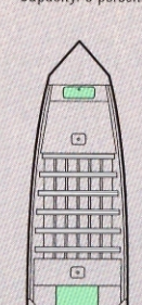
MV 1544 AW DD 15' Length 46" Bottom/65" Width 25 HP maximum Weight: 260# Hull thickness: .082" Capacity: 4 persons
