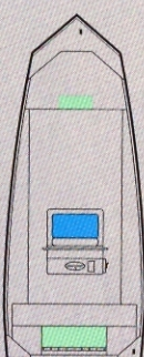
MV 1860 AW CC 18' Length 60" Bottom/86" Width 90 HP maximum Weight: 780# Hull thickness: .102" Capacity: 6 persons
