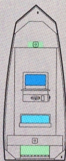
MV 1860 AW FF 18' Length 60" Bottom/86" Width 90 HP maximum Weight: 780# Hull thickness: .102" Capacity: 6 persons
