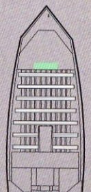
V-Bow 1650 AW Tunnel 16' Length 50" Bottom/74" Width 35 HP maximum Weight: 450# Hull thickness: .102" Capacity: 5 persons
