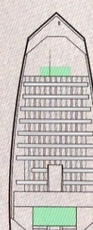
V-Bow 1860 AW Tunnel 18' Length 60" Bottom/86" Width 50 HP maximum Weight: 795# Hull thickness: .102" Capacity: 6 persons
