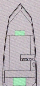
MV 1650 SC 16' Length 50" Bottom/74" Width 60 HP maximum Weight: 575# Hull thickness: .102" Capacity: 5 persons
