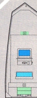
MV 2072 AW Tunnel FF 20' Length 72" Bottom/96" Width 115 HP maximum Weight: 1100# Hull thickness: .102" Capacity: 8 persons
