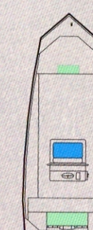
V-Bow 1860 AW Tunnel CC 18' Length 60" Bottom/86" Width 90 HP maximum Weight: 795# Hull thickness: .102" Capacity: 6 persons
