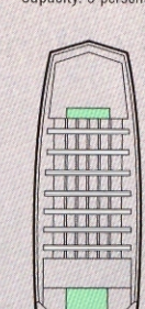
MV 1544 AW 15' Length 46" Bottom/65" Width 25 HP maximum Weight: 250# Hull thickness: .082" Capacity: 4 persons
