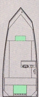
MV 1860 SC 18' Length 60" Bottom/86" Width 90 HP maximum Weight: 780# Hull thickness: .102" Capacity: 6 persons
