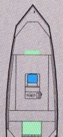
MV 1650 AW CC 16' Length 50" Bottom/74" Width 60 HP maximum Weight: 575# Hull thickness: .102" Capacity: 5 persons
