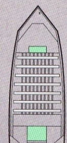
MV 1650 AW 16' Length 50" Bottom/74" Width 40 HP maximum Weight: 450# Hull thickness: .102" Capacity: 5 persons
