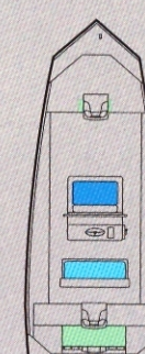
V-Bow 1860 AW Tunnel Spl 18' Length 60" Bottom/86" Width 90 HP maximum Weight: 795# Hull thickness: .102" Capacity: 6 persons
