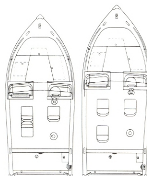
Comb-Pedestal Seating Pedestal Seating Trophy 170 Shown
