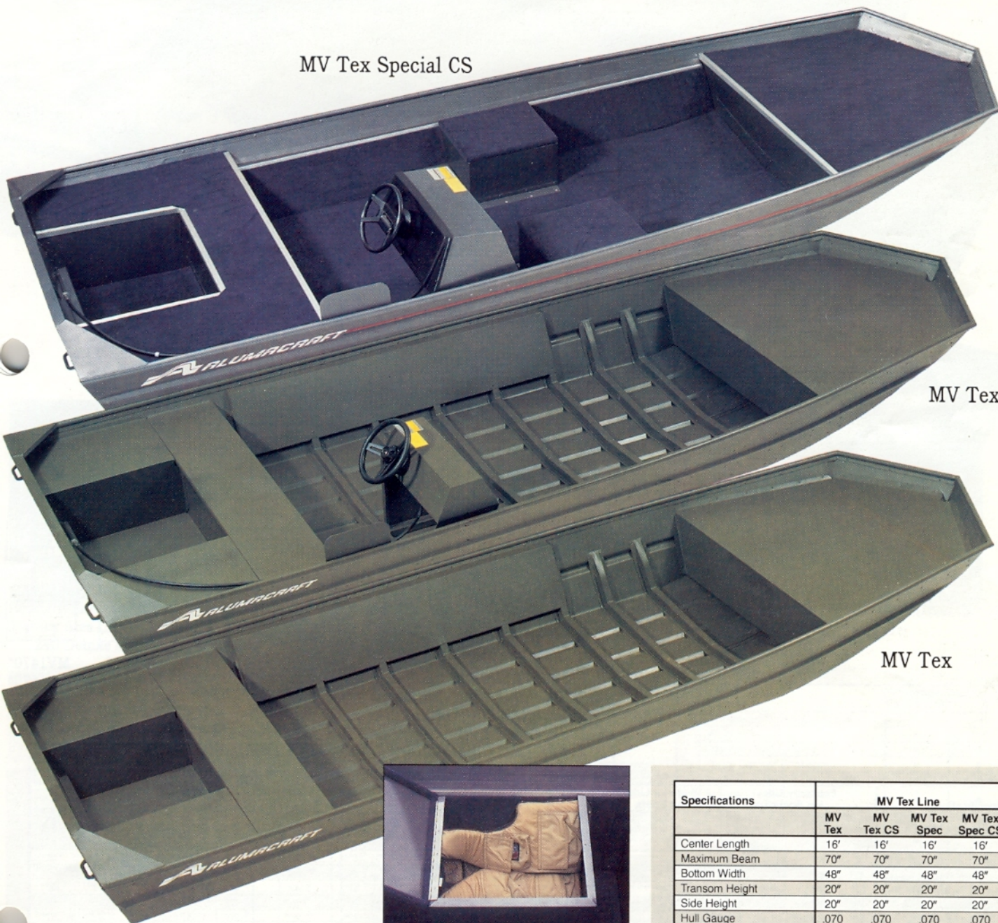
Optional Camouflage Upholstered Seat and Clamp
