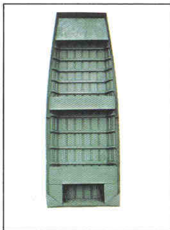
*1470-*1670-1870 Beam 70" — Bottom width 48" — HP range: 1470 10-25 HP, 1670 15-35 HP, 1870 15-40 HP — *Livewell model available.
