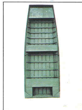
1474-1674-1874 Beam 74" — Bottom width 52" — HP range: 1474 15-30 HP, 1674 15-35 HP, 1874 15-40 HP
